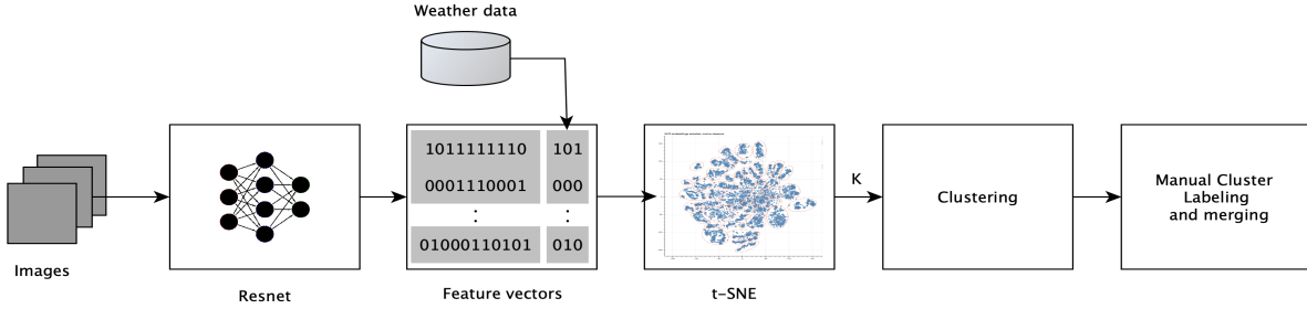
Figure 2: The overall architecture of our workflow is shown. Images are fed into a ResNet model to obtain feature vectors. The features are then combined with weather data. Using t-SNE we find the potential number of clusters in the data and then perform clustering using KMeans. The resulting clusters are then manually labeled and merged. The workflow is implemented using Keras, Python3, HTML, and Javascript. We used a Quadro M6000 GPU for generating the ResNet feature vectors.
