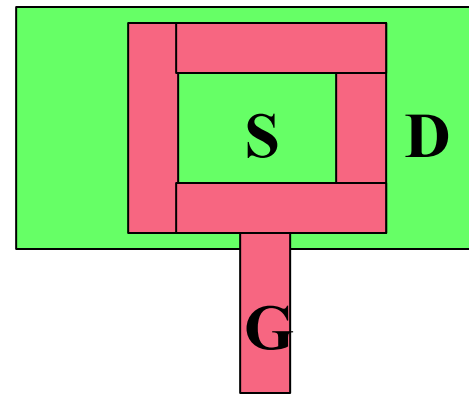
Radiation-Tolerant Layout
