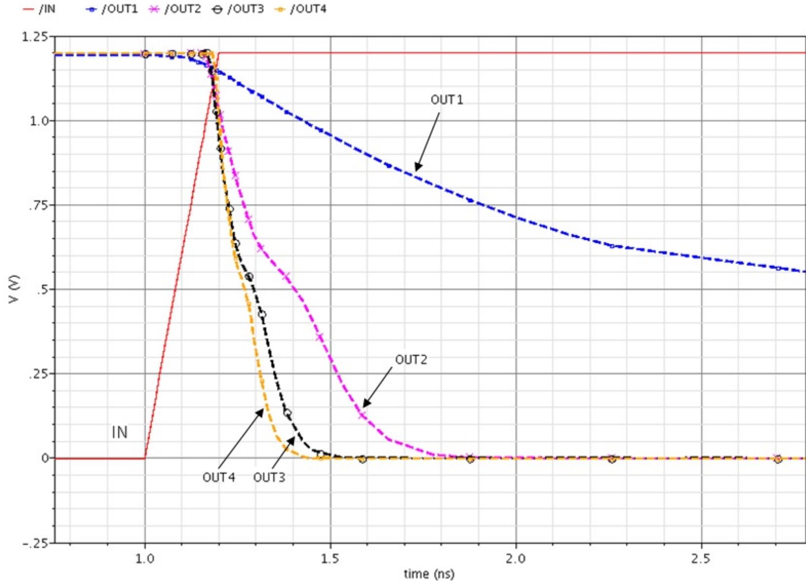
Transient Response
