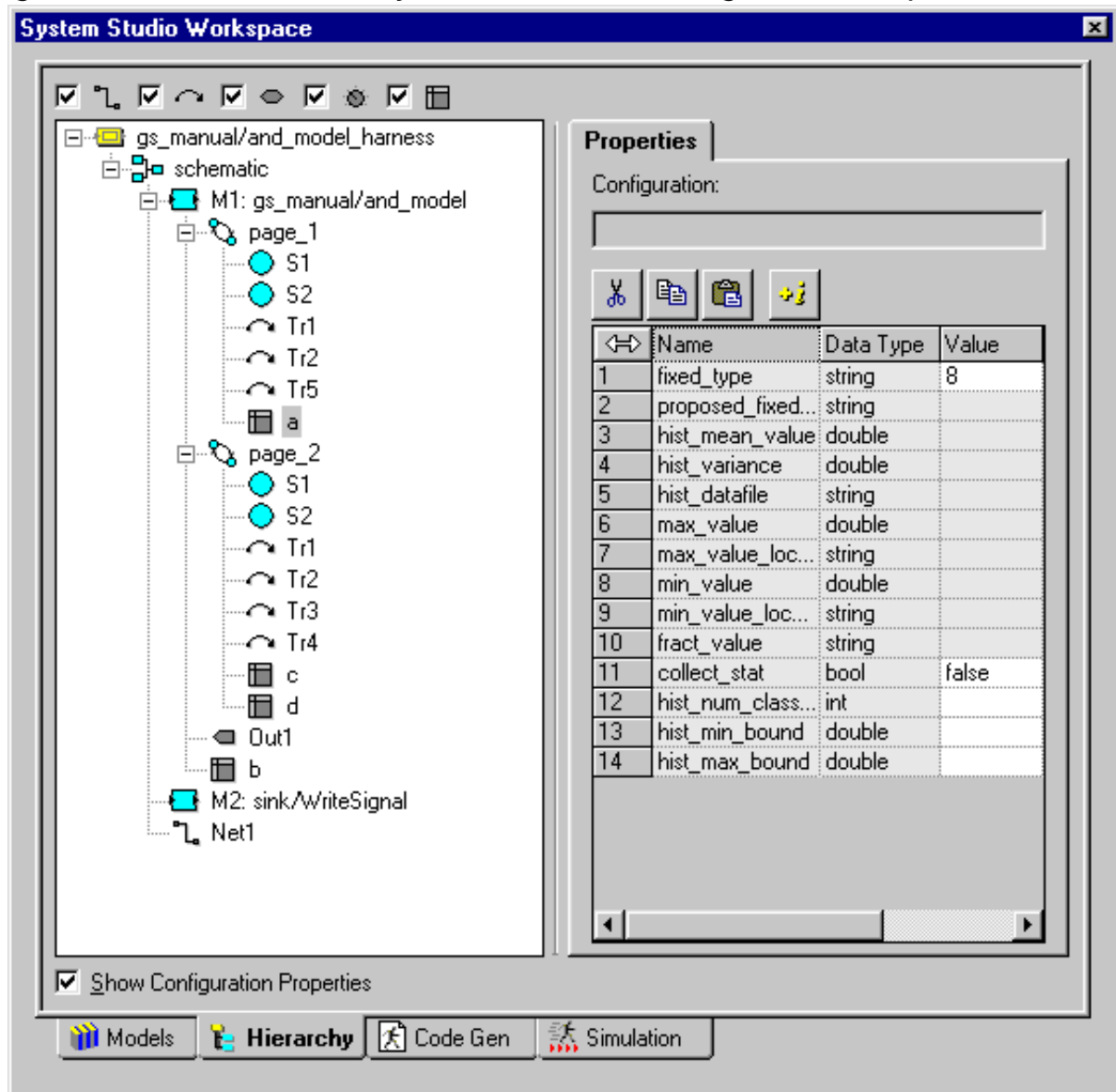
Figure 2-17 The Hierarchy Browser, with Configuration Properties
