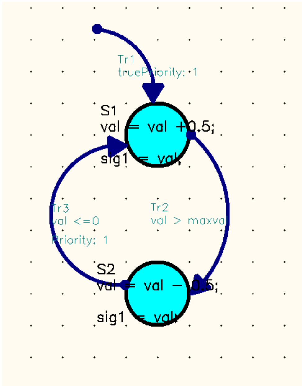
Figure 6-9 The Completed FSM Model in Page 1
