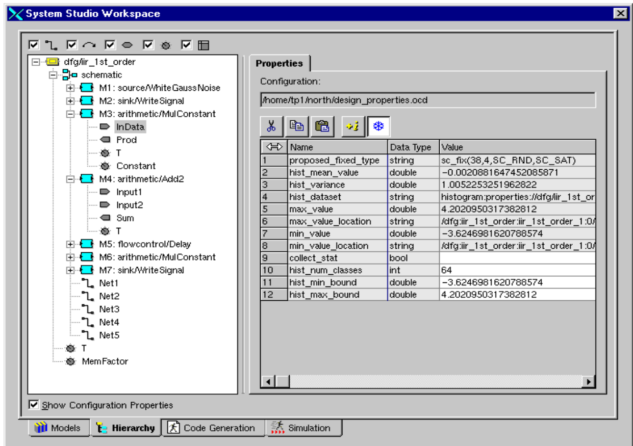
Figure 8-4 The Configuration Properties after Merging
