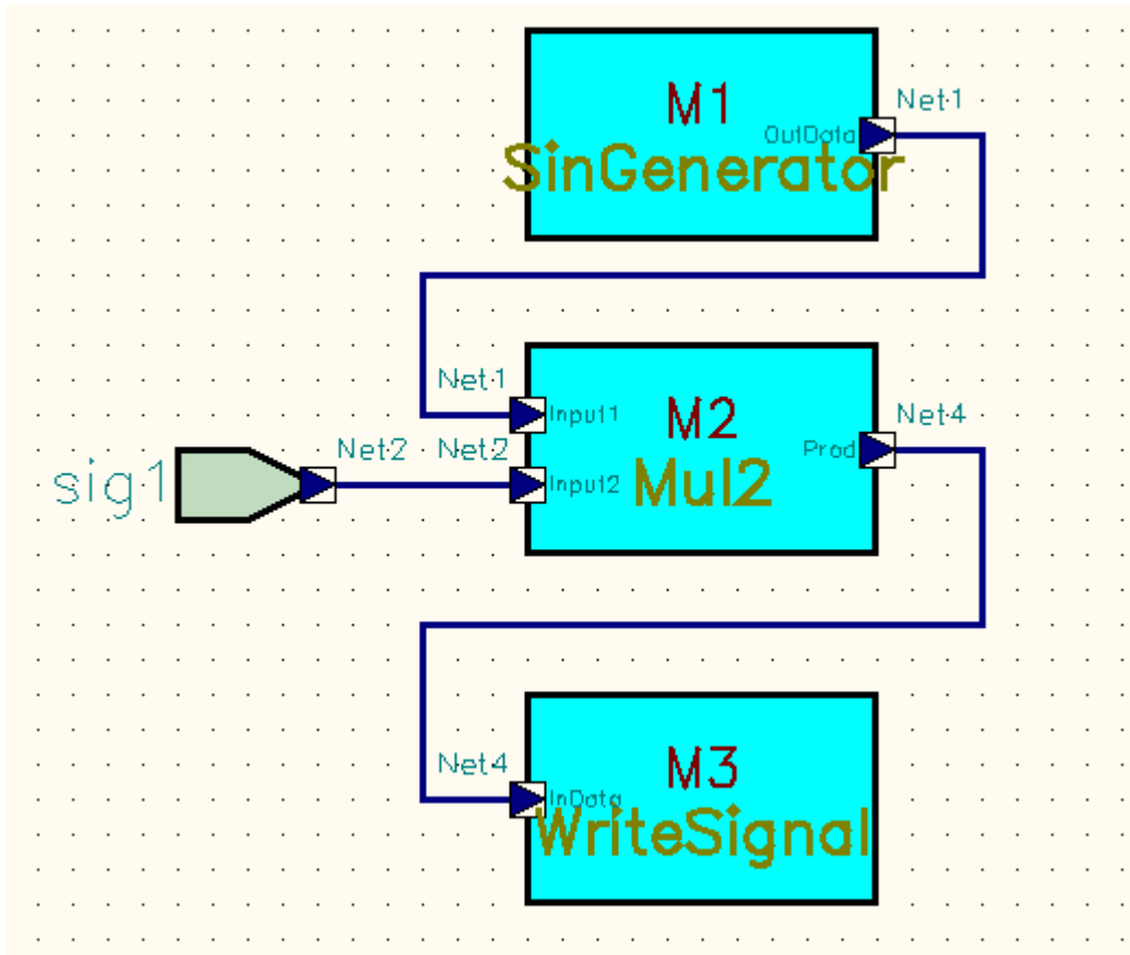
Figure 6-13 The Completed DFG
