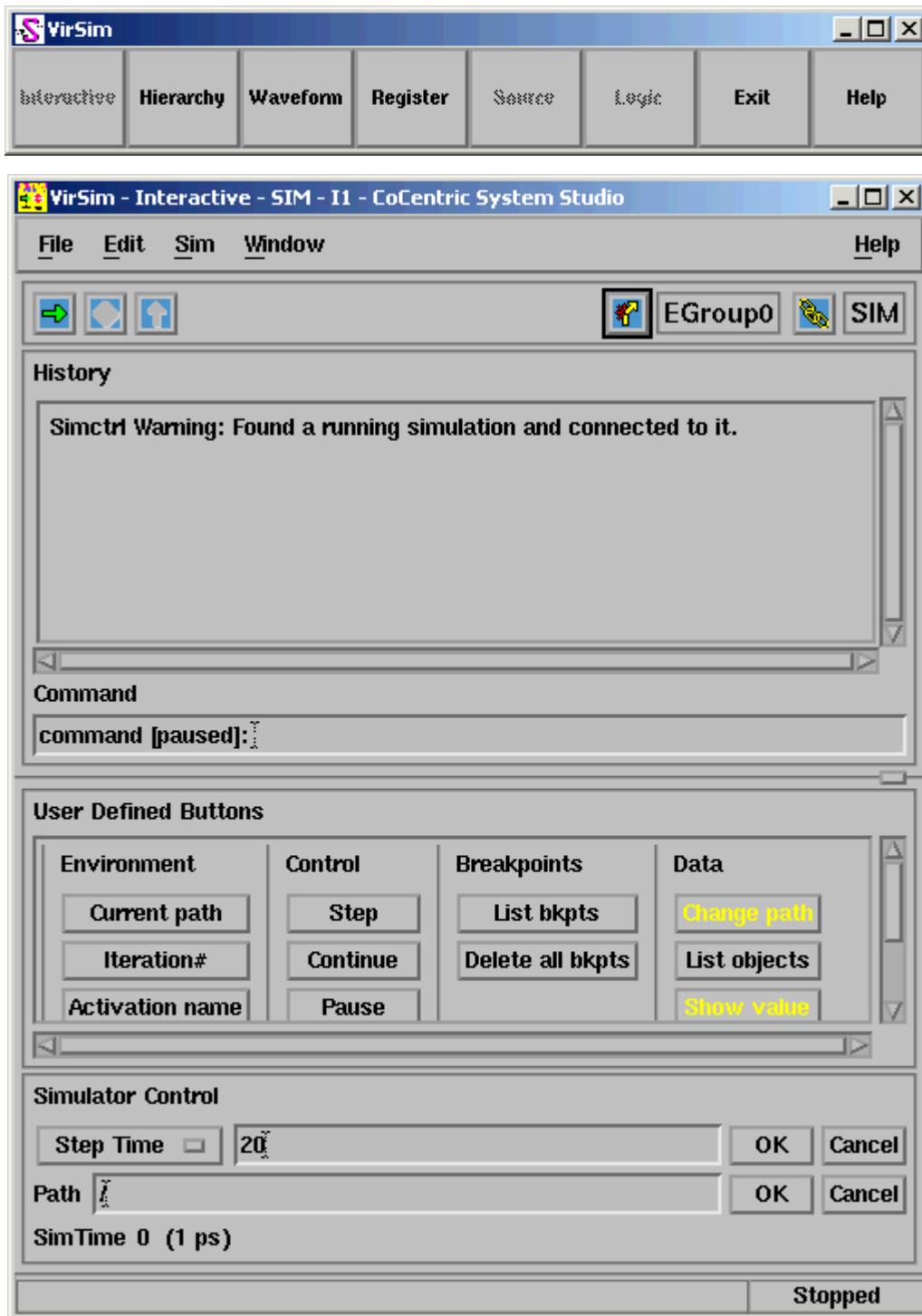
Figure 7-28 VirSim Main Menu and Interactive Window
