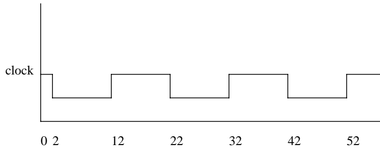
FIGURE 3. Offset Clock Waveform
