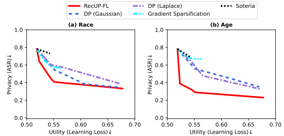
Figure 3: Multi-attribute protection on LFW.
