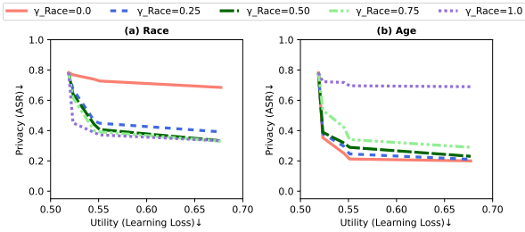
Figure 4: Multi-attribute protection with varying \gamma on LFW.
