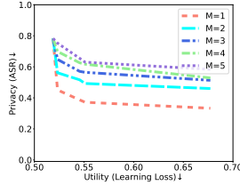
Figure 5: Multi-attribute protection with varying M on LFW. vulnerable. A similar trend can be observed on the age attribute in Figure 4(b). We also notice that even with the \gamma_{race} = 0 , the ASR of the race inference attack would still drop slightly when a large perturbation is used. Therefore, even when RecUP-FL is set to focus on a particular attribute, it still has a certain degree of effect over other attributes due to the correlation between these attributes.
