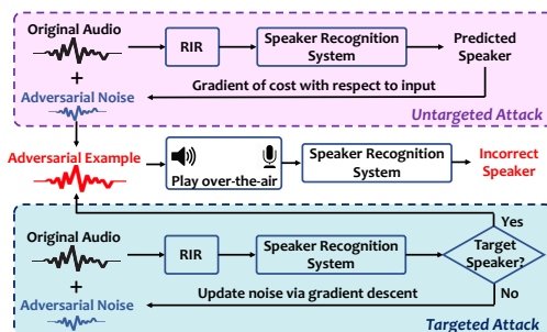
Figure 2: Attack overview.
