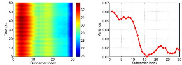
(a) CSI time series patterns (b) Variance of each subcarrier after data calibration.
