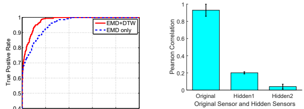
Figure 16: Similarity between the vibrations received by VibWrite's original receiver and hidden receivers.
