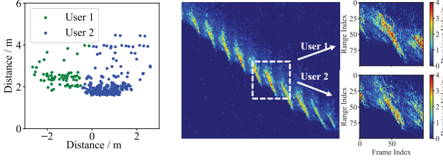
Fig. 7: Scatters of two abreast users in the spatial domain. (left), and separation results (right).
