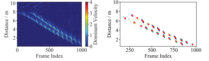
(a) Lower limb motion map of two users walking towards the radar. (b) Step segmentation clustering result with step center marked as red.
