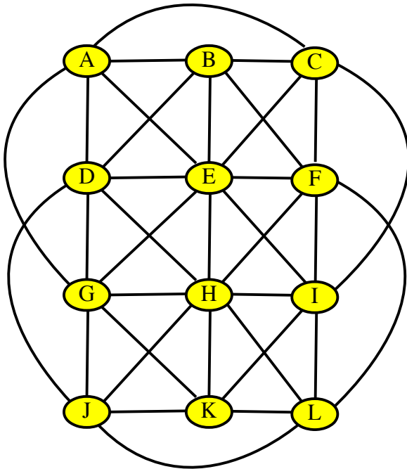
Graph Structure
