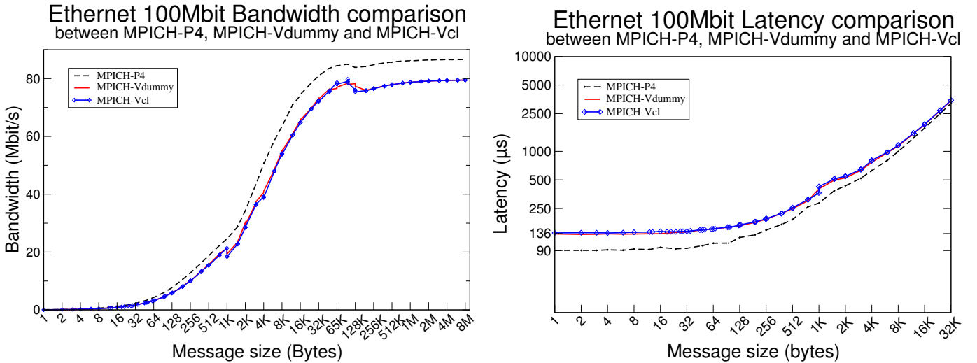
Fig. 7. Bandwidth and latency comparison between MPICH-P4, MPICH-Vdummy, and MPICH-Vcl on Fast-Ethernet network.
