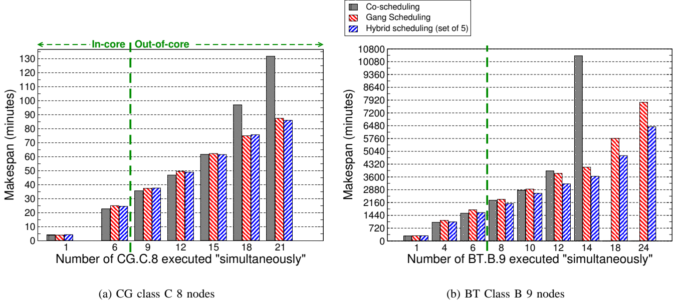
Fig. 11. Makespan for n simultaneous applications using Co-scheduling, Gang scheduling or hybrid scheduling.
