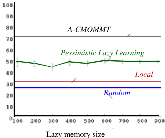
Figure 5. Performances of the Pessimistic lazy Q-learning approach compared to a random action selection policy, a user-defined non-cooperative policy and the hand-generated solution A-CMOMMT , for 10 robots and 10 randomly moving targets. The results are the mean of 10 different experiments per point for lazy learning policy, and 100 experiments for the other 3 policies. Each experiment duration is 1000 iterations.
