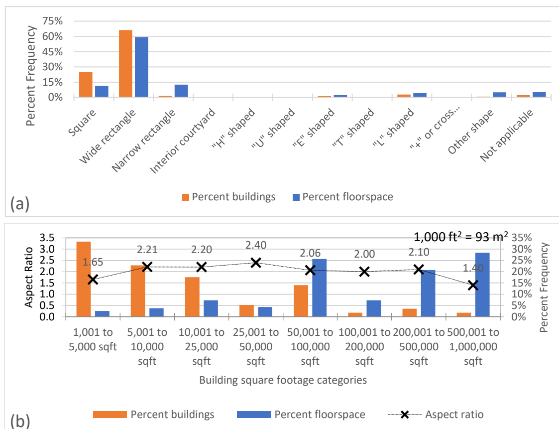
Figure 13. Building shape statistics for (a) courthouses in the 2012 CBECS data [41] and (b) 'Public Order and Safety' buildings in the 1992 CBECS data [47].
