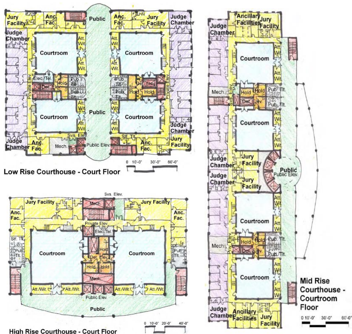
Figure 4. Example floor plan for courtroom floors of low-rise, mid-rise and high-rise federal courthouses [34].
