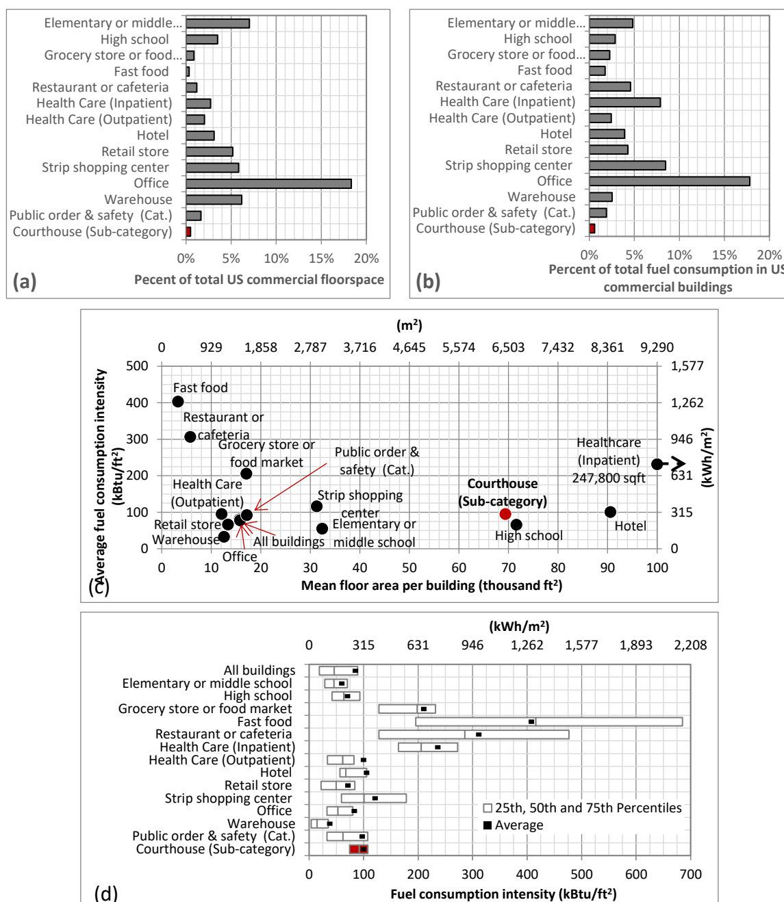
Figure 1. Courthouses in the US commercial building stock [41]. Courthouses account for 0.5% of US commercial floorspace (a); 0.6% of fuel consumption in US commercial buildings (b); are dissimilar to most other buildings in terms of average floor area but comparable in terms of average fuel consumption intensity (c) and have a narrower range of variation of fuel consumption intensity compared to most other building types (d).
