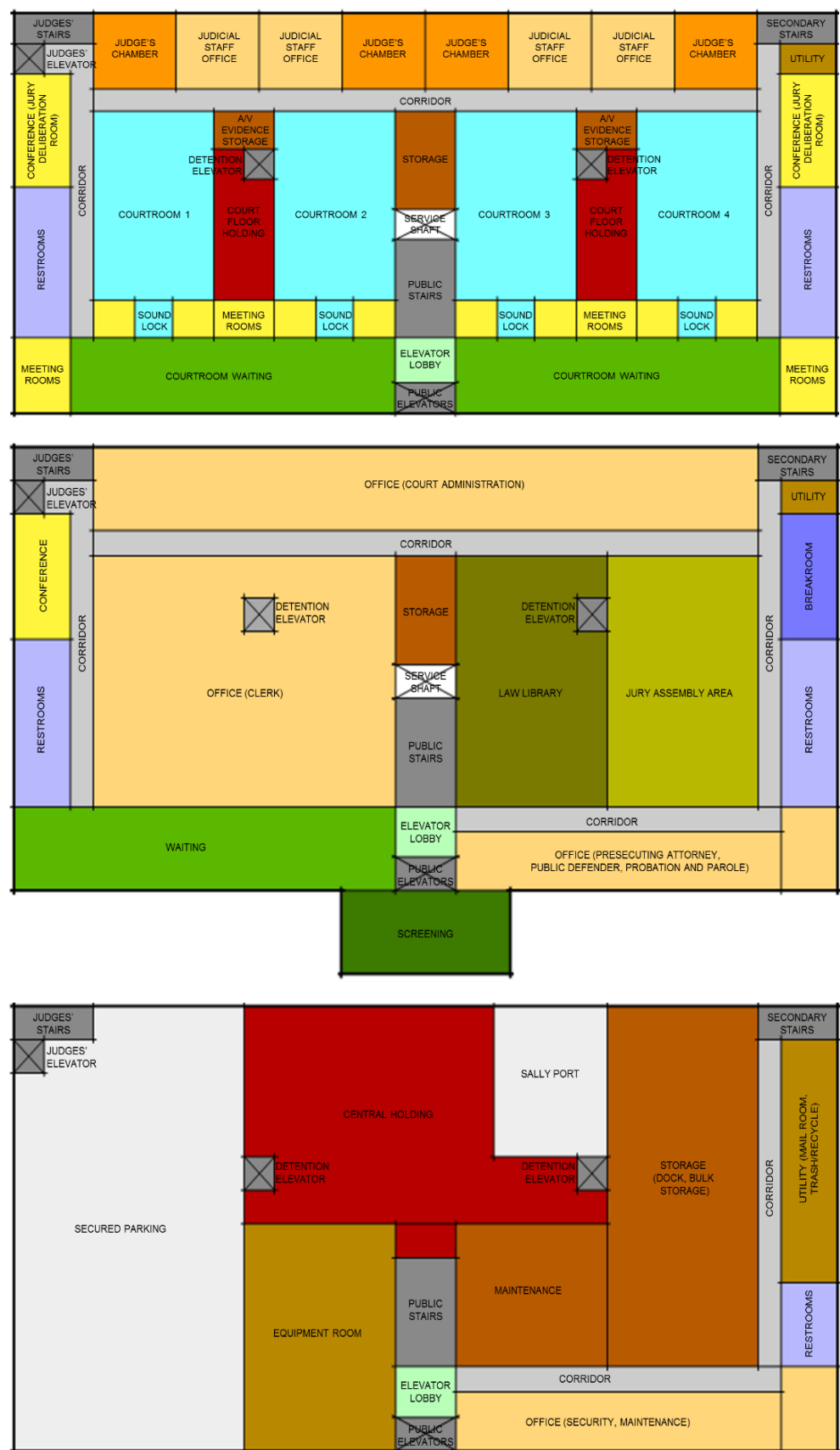
Figure 17. Prototype courthouse layout of basement ( bottom ), first floor ( middle ) and second floor ( top ). Error! Reference source not found. shows the usable space area distribution for the prototype courthouse and confirms the suitability of the proposed area programming when compared to Error!
