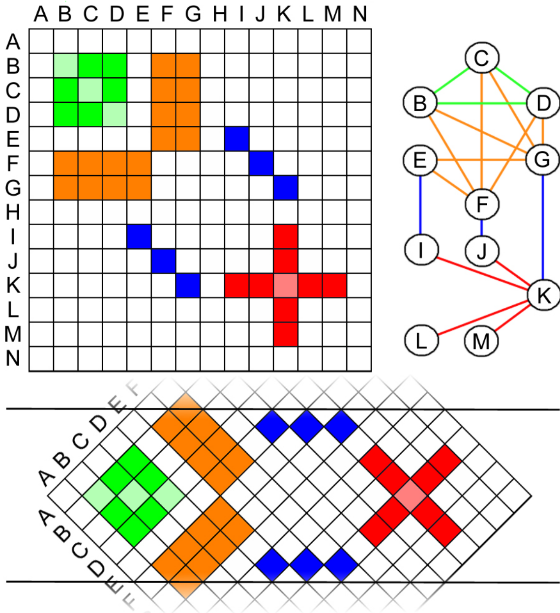
Figure 3.2: Illustration of a permuted adjacency matrix with common graph patterns (top), and extraction of the BTD belt for qualitative selection (bottom).
