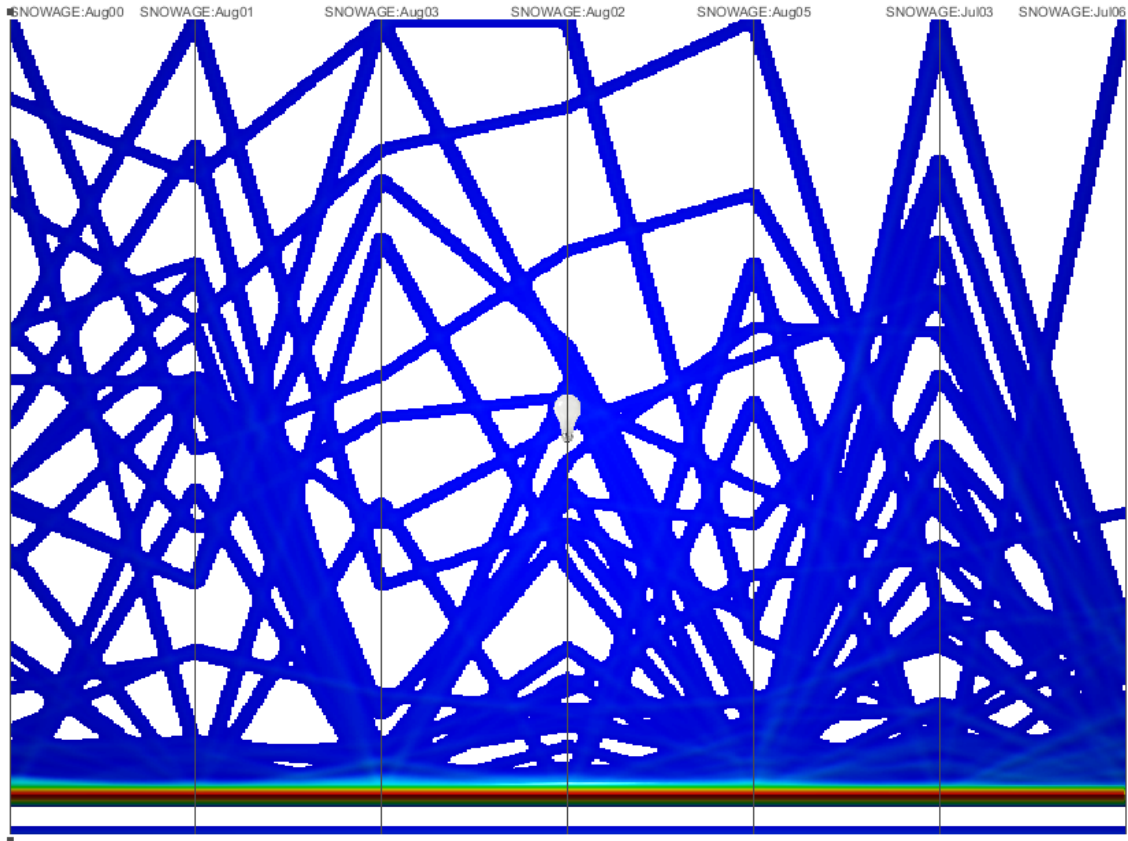
Figure 4.9: An image-space metric quantifying open space finds that age of visible snow is typically low but with slightly increased age in July'03.
