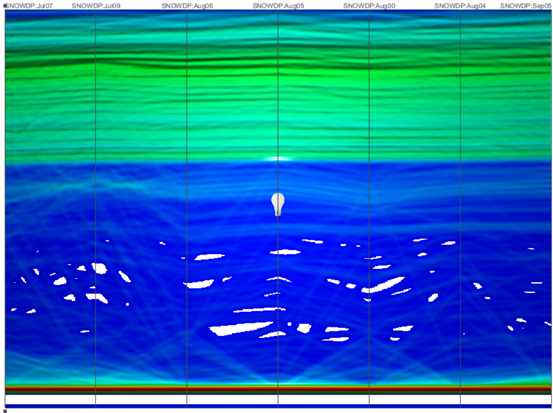
Figure 4.8: One way of measuring global warming showing strong correlation of snow depth between years. Our rendering technique also shows V-shaped highlights corresponding to grid locations that my warrant further investigation for snow/ice melting.
