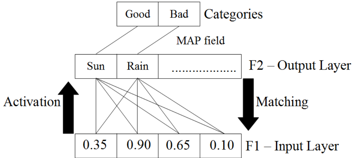
Figure 5.3: Structure of an ARTMAP network.
