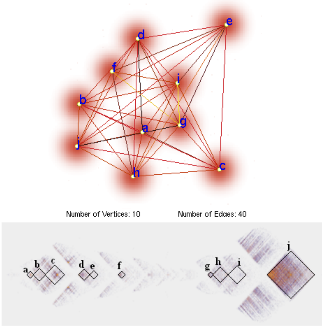
Figure 3.4: A 2D level-of-detail graph created from brushed BTM belt selections to show correlations among BTM structures.
