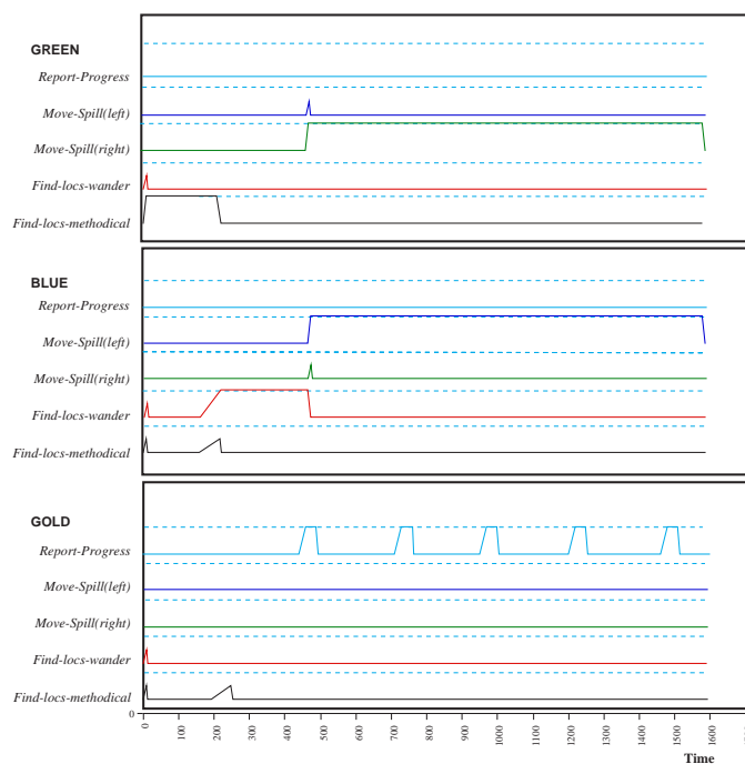
Fig. 14. Motivational levels for behavior sets during experiment with spill finding error. The dashed lines represent the thresholds of activation of each behavior set.
