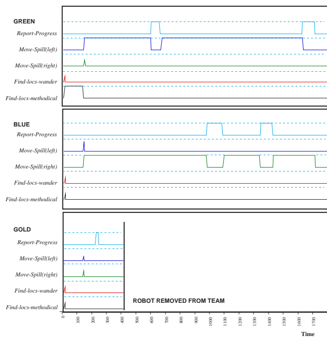
Fig. 22. Motivational levels for behavior sets during experiment when a team member that is reporting the progress is removed. The dashed lines represent the thresholds of activation of each behavior set.
