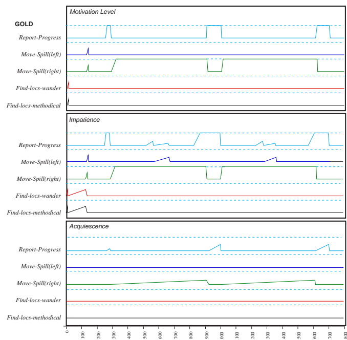
Fig. 20. Motivational, impatience, and acquiescence levels for behavior sets of GOLD during experiment when a team member that is moving a spill is removed. The dashed lines represent the thresholds of activation.
