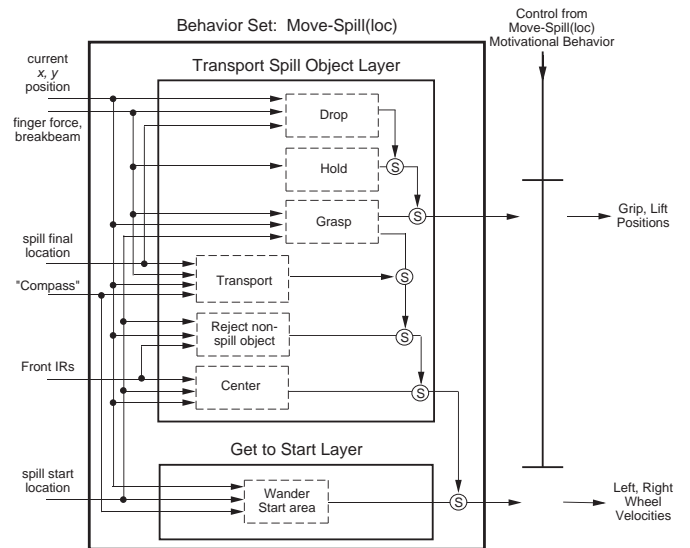
Fig. 7. The robot control organization within the move-spill(loc) behavior set.
