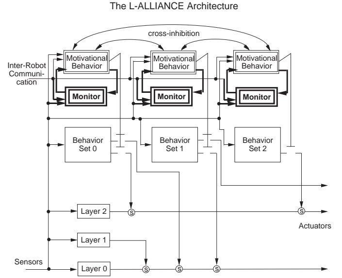
Fig. 2. The L-ALLIANCE architecture, which adds in the capability for dynamic parameter adaptation.
