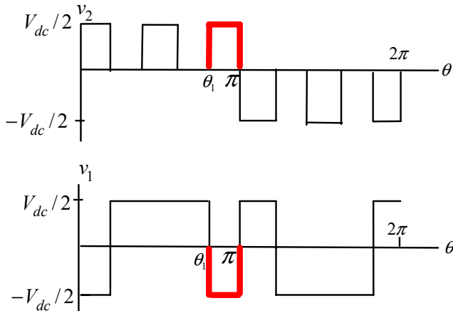
Fig. 4. Another way to make the output voltage zero for \theta_1 \leq \theta \leq \pi is to set v_1 = -V_{dc}/2 and v_2 = +V_{dc}/2 .
