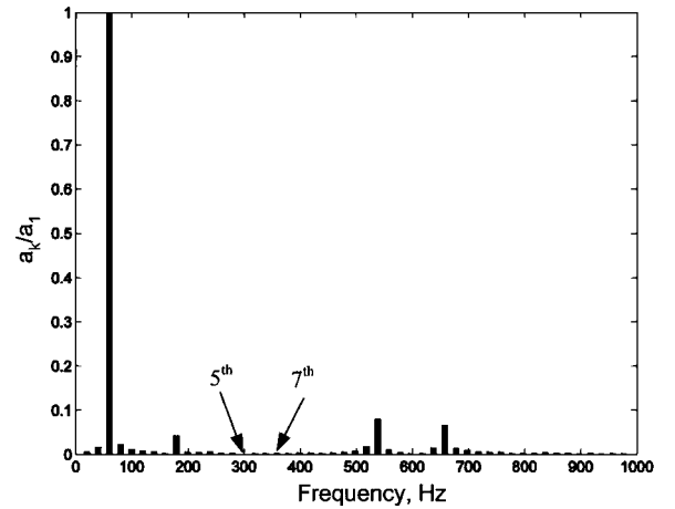
Fig. 5. Normalized (with respect to the fundamental) FFT versus frequency.
