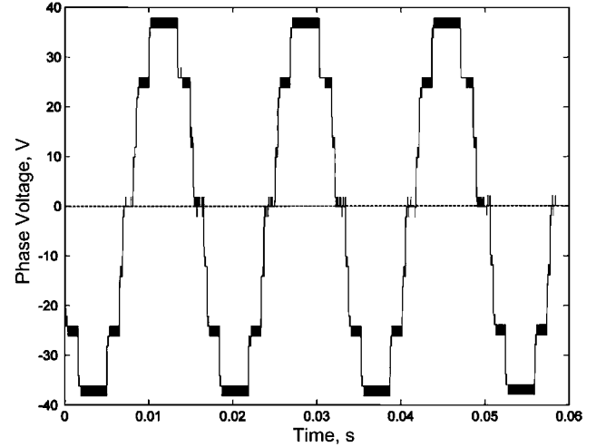
Fig. 4. Experimental output voltage waveform.
