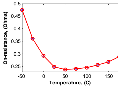
Fig. 11. On-resistance of SiC MOSFET at different temperatures.
