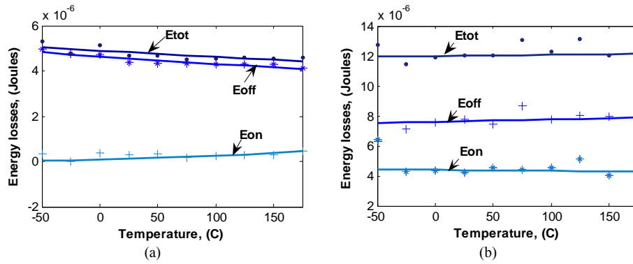
Fig. 17. Energy loss plots for (a) VJFET, (b) MOSFET.
