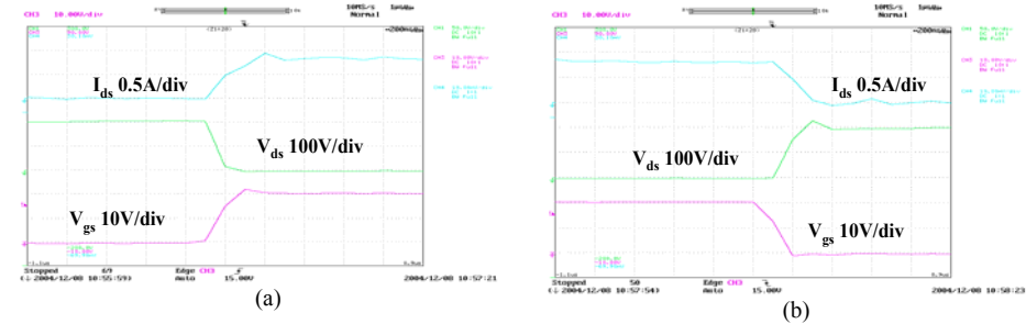
Fig. 16. The gate and switching waveforms of the SiC MOSFET.
