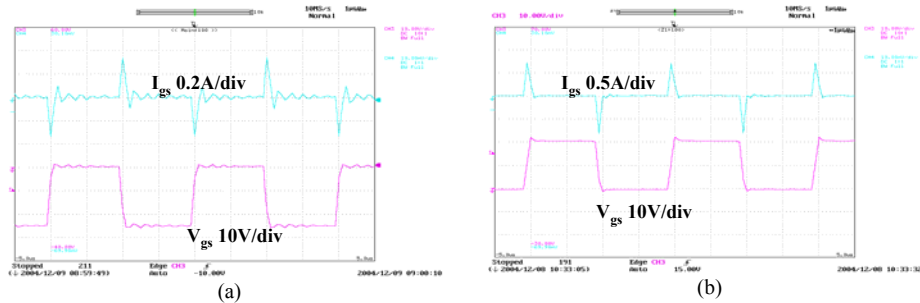
Fig. 14. The peak gate currents and gate voltage waveforms with (a) SiC VJFET, (b) SiC MOSFET.
