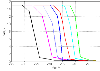
Fig. 8. Transfer characteristics of several SiC VJFET samples.
