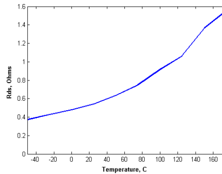
Fig. 7. On-resistance of SiC VJFET at different temperatures.
