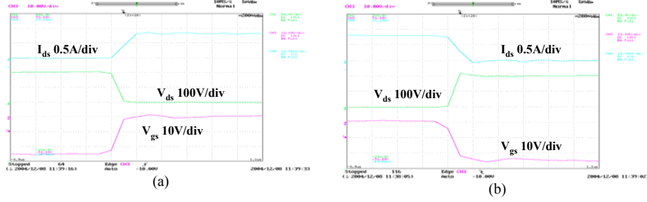
Fig. 15. The gate and switching waveforms of the SiC VJFET.
