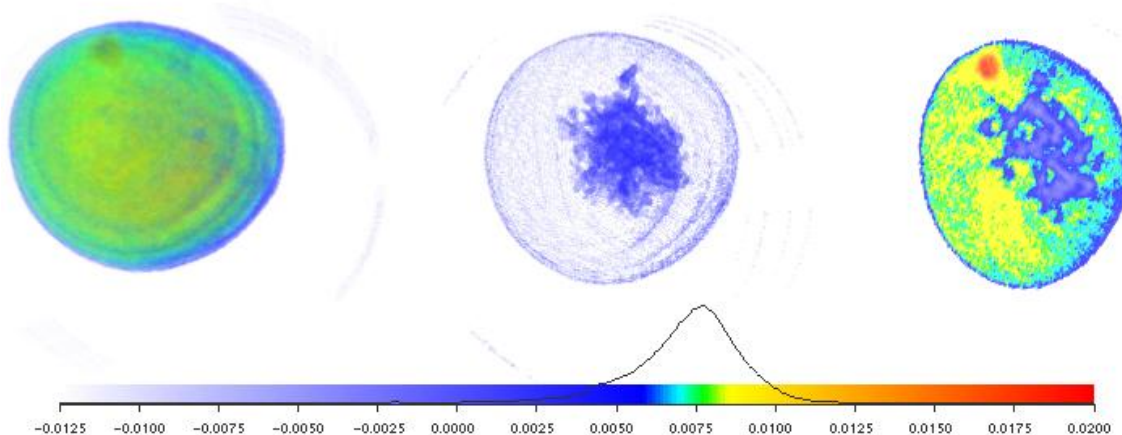
Figure 3: Multiview visualization of a meteorite’s porous space. After filtering the data associated with air (see Figure 2) we study the meteorite’s porous space. From left to right: (1) volume visualization of the filtered data; (2) volume visualization of range 0.001 – 0.005 (the porous space); (3) a slice through the center of the high-attenuation core (see Figure 2).
