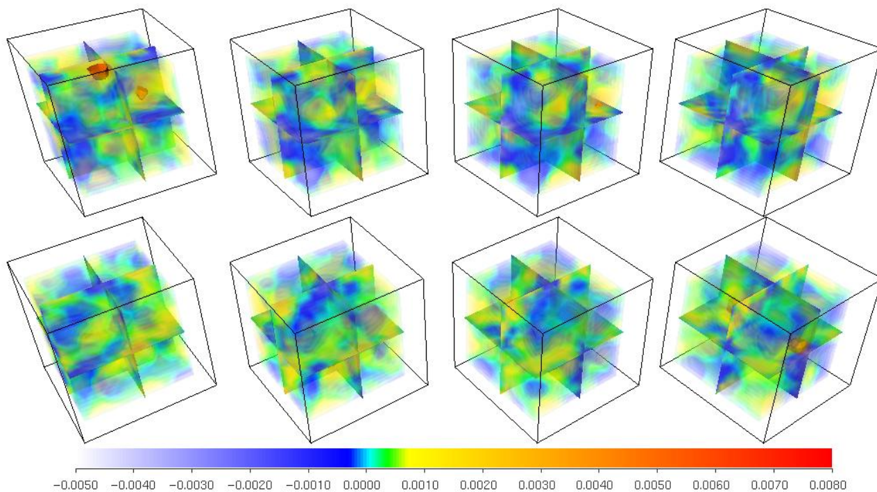
Figure 1: Multiview visualization of QCD data. Shown is topological charge density on a 4D xyzt lattice of size 16 \times 16 \times 16 \times 16 . We show volume visualization of slices for t = 1, \dots, 8 . The ordering is from left to right, top to bottom. There is one iso-surface at 0.005.
