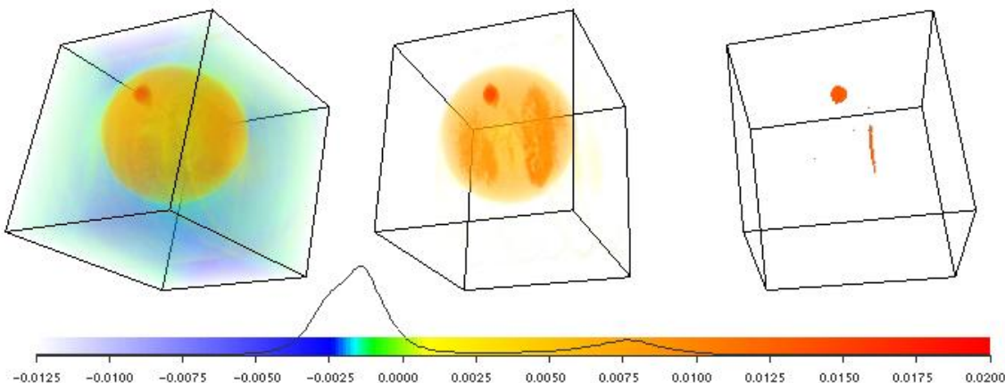
Figure 2: Multiview visualization of a meteorite’s core. From left to right: (1) volume visualization of the whole data; (2) volume visualization of data range 0.002 – 0.02; (3) volume visualization of range 0.0125 – 0.02. Used in studies for the presence and the relative location of different metals that correspond to different attenuation ranges of the data.
