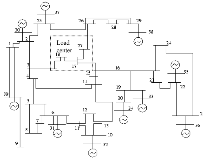
Figure 1. New England test system
