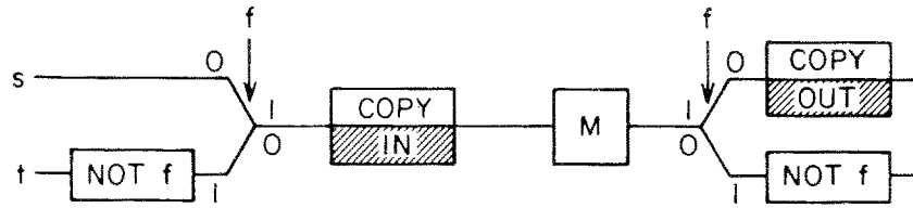
Figure III.41: Garbage clearer. 0/1 annotations on the wires show the f values. [fig. from F85]
