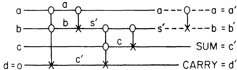
Figure III.38: Simple adder using reversible logic. [fig. from F85]
