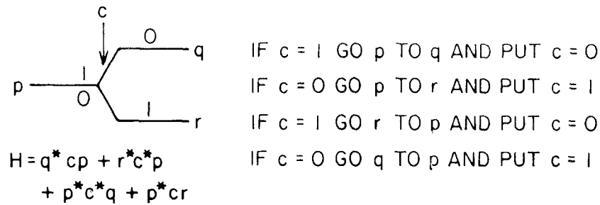
Figure III.39: Switch element. 0/1 annotations on the wires show the c values. [fig. from F85]
