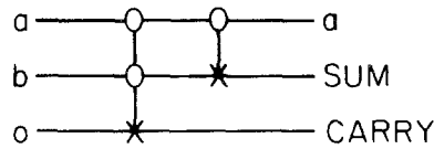
Figure III.37: Simple adder using reversible logic. [fig. from F85]
