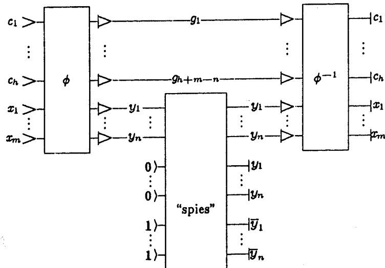
Figure II.17: Garbageless circuit. (Fredkin &amp; Toffoli, 1982)
