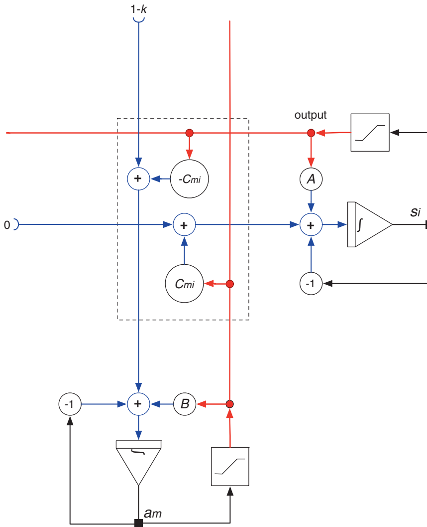
Analog Computation, Fig. 1 Analog program for Boolean satisfiability
