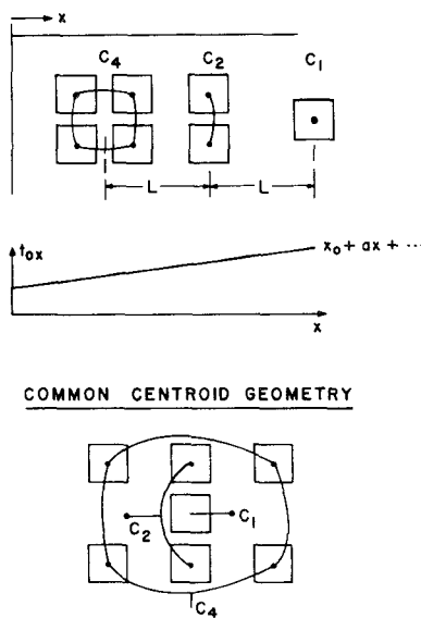
Fig. 7. Capacitor ratio error due to oxide gradients.
