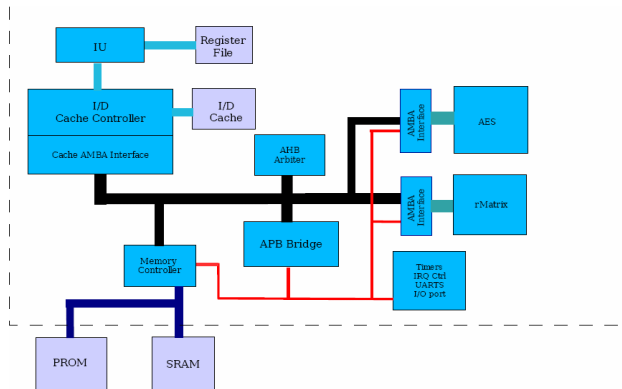
Figure 1. SoC Platform Block Diagram
