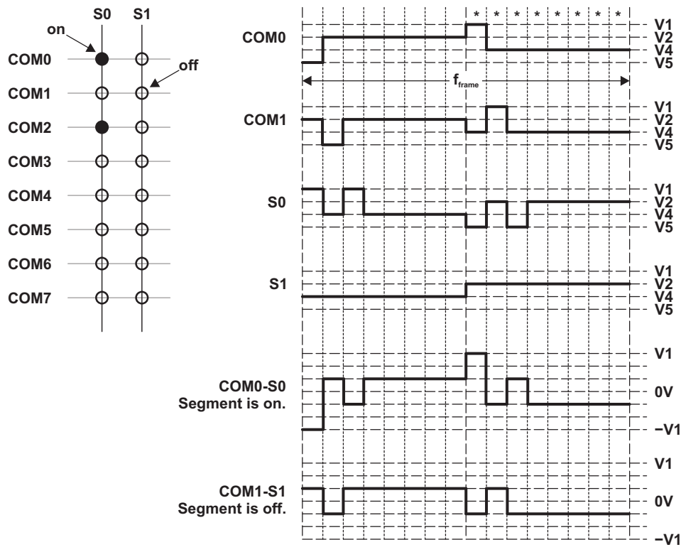
Figure 35-11. Example 8-Mux, 1/3 Bias Low-Power Waveforms (LCDLP = 1)
