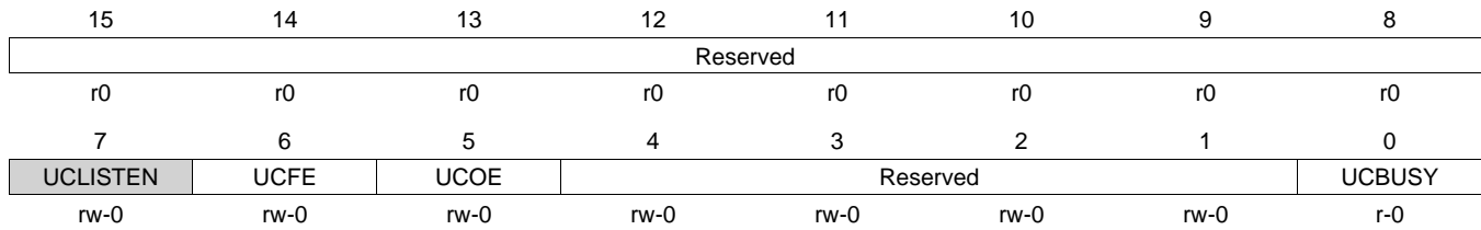
Figure 40-7. UCxSTATW Register
