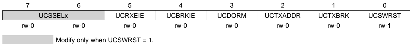
Figure 36-13. UCAXCTL1 Register
