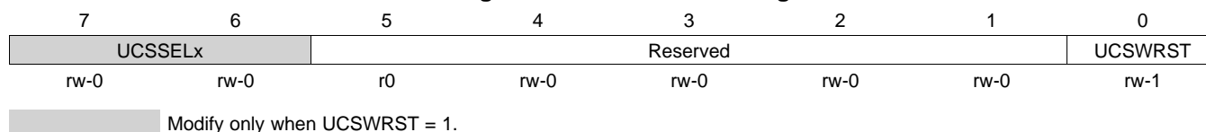
Figure 37-17. UCBxCTL1 Register
