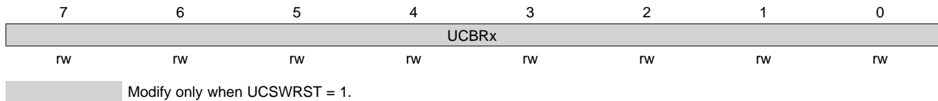
Figure 38-19. UCBxBR0 Register
