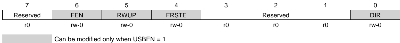
Figure 42-27. USBCTL Register
