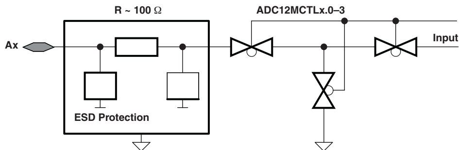
Figure 28-3. Analog Multiplexer
