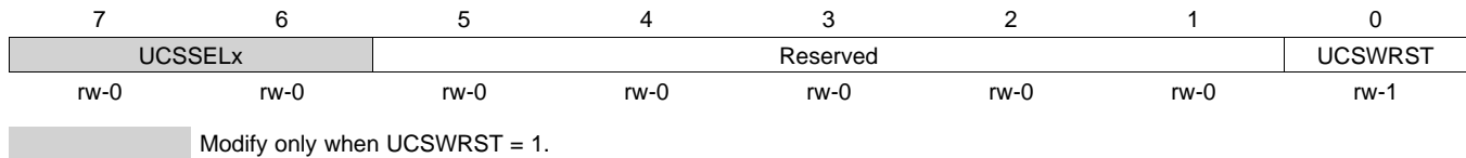
Figure 37-6. UCxCTL1 Register
