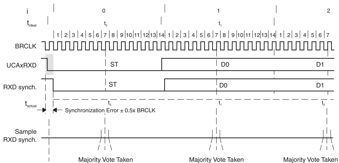
Figure 36-11. Receive Error
