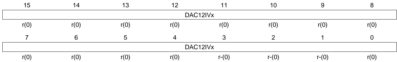
Figure 31-20. DAC12IV Register
