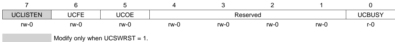
Figure 37-10. UCxSTAT Register
