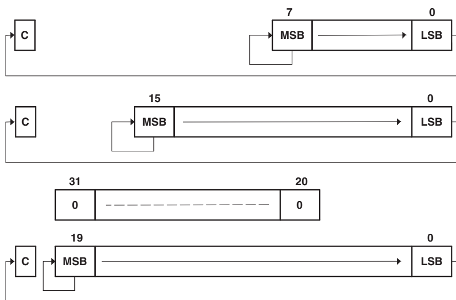
Figure 6-49. Rotate Right Arithmetically RRAX(.B,.A) – Non-Register Mode
