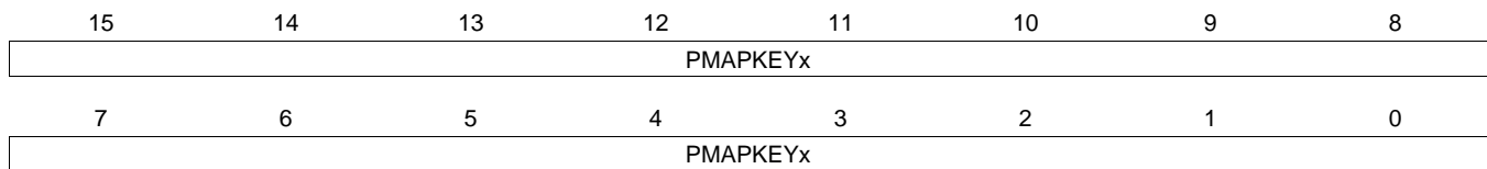
Figure 13-1. PMAPKEYID Register
