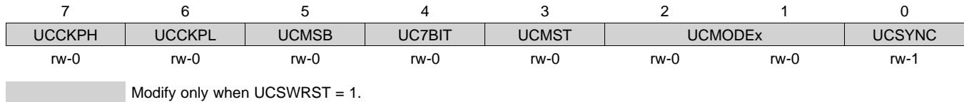
Figure 37-16. UCBxCTL0 Register
