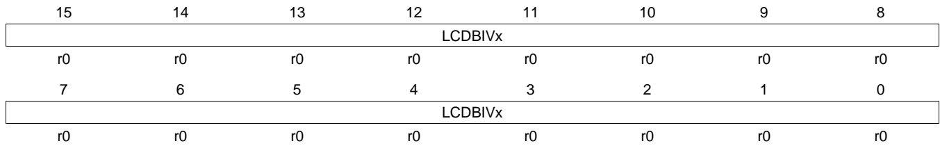
Figure 34-22. LCDBIV Register
