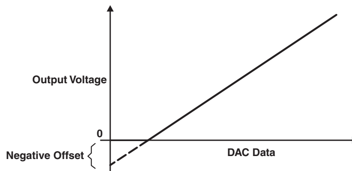
Figure 31-5. Negative Offset
