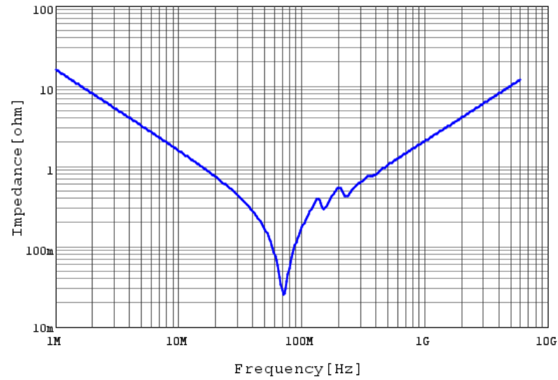
GRT1885C1H103JA02 |Z| DCOV, 25degC
