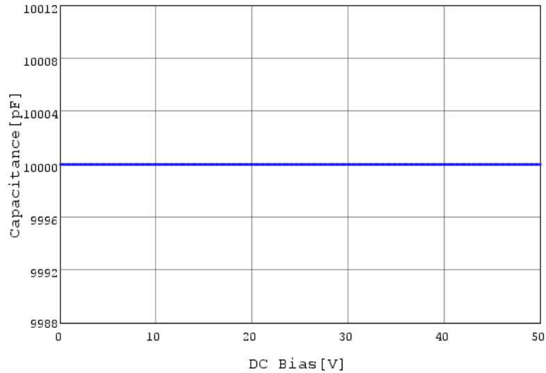
GRT1885C1H103JA02 C-DC bias capacitance, 25.0degC, AC1Vrms
