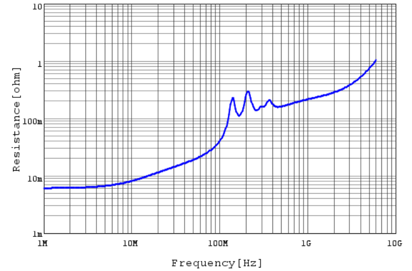
GRT1885C1H103JA02 R DCOV, 25degC
