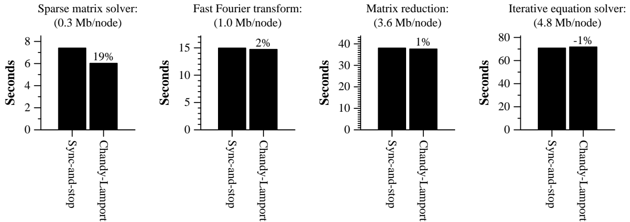
Figure 5. Overhead of sync-and-stop vs. Chandy-Lamport on the Intel iPSC/860. Although sync-and-stop is more primitive and freezes all the processors, it does not degrade performance significantly in most applications.
