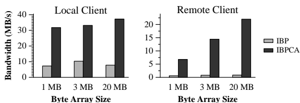
Figure 6. Performance of ibpca_store_block() with duplicate files from local and remote clients.
