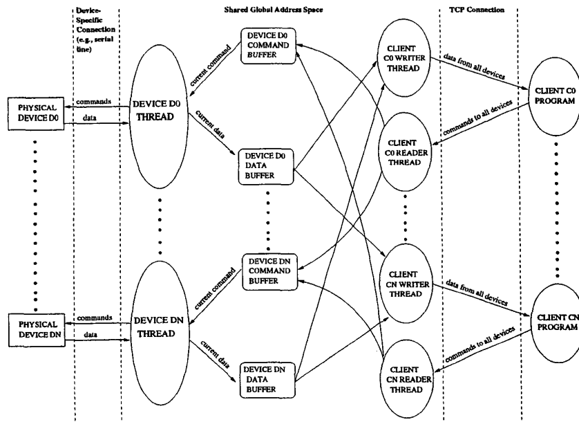
Figure 2: Overall system architecture of Player
