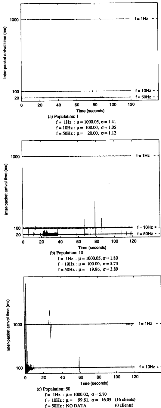
Figure 3: Inter-packet arrival times measured while serving large amounts of sensor data across wireless Ethernet to different client populations.
