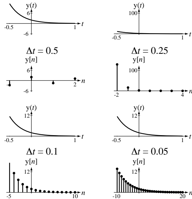
Figure Q-2 Solution of the first-order, linear, constant coefficient, ordinary difference equation approximating a differential equation for four different choices of \Delta t
