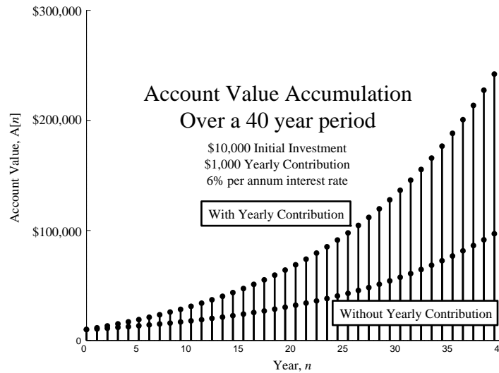
Figure Q-4 Account value accumulation over a 40 year period with $10,000 initial investment at 6% interest compounded annually, with and without $1,000 per year contribution
